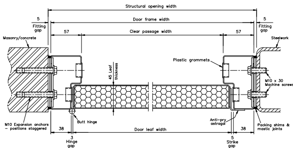
Sunray Single ExcluDoor® 1 FR
